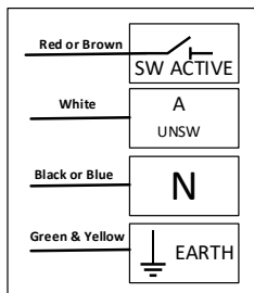
Emergency & Mains Wiring Connections
