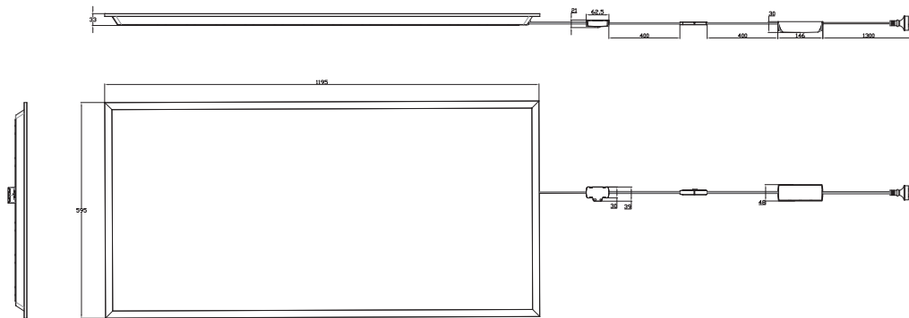
ECOP126CSEG2 – 1195 mm x 595 mm x 30.3mm
