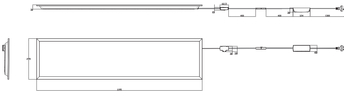
ECOPL123CSEG2/ECOPL1234UG19/ECOPL1234EG2 – 1195 mm x 295 mm x 30.3mm
