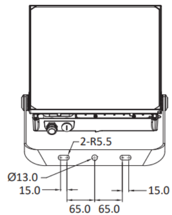
Trunnion arm dimension drawing with all mounting holes
