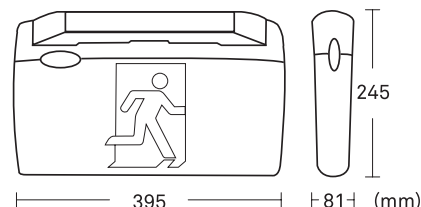
AQUA LOCK-W (IP65) with LED Stingray
