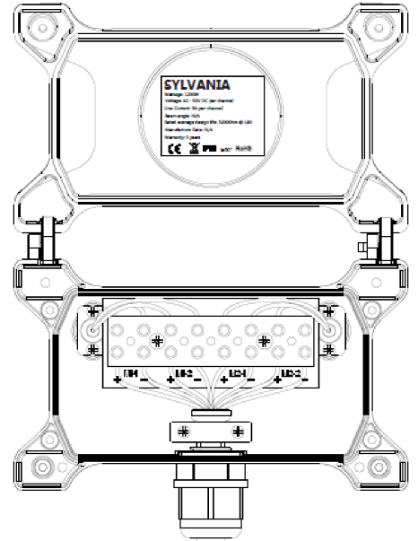
Junction Box
