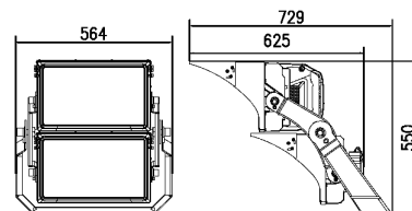
1200W dimensions
