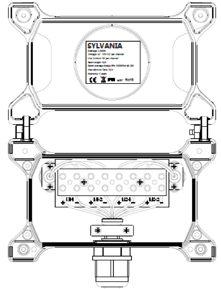
Junction Box
