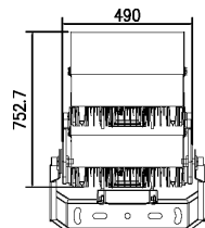
1200W Maximum projected dimensions
