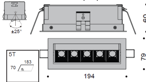
NANO 11W Cut out: 70 x 183 (mm)
