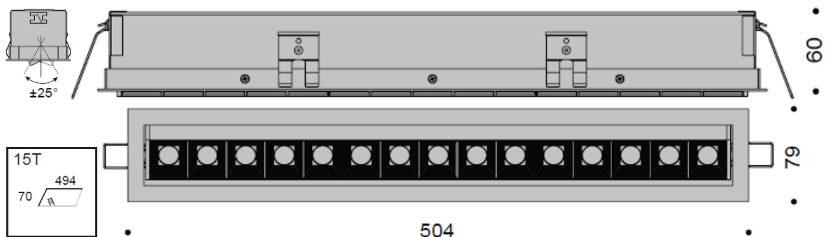
NANO 33W Cut out: 70 x 494 (mm)
