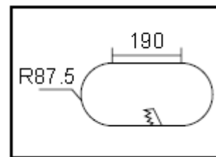
JAX EYE 40W TWIN Cut out: R87.5 x 190 (mm)
