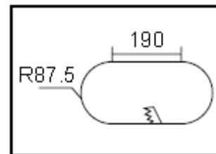
JAX EYE 30W TWIN Cut out: R87.5 x 190 (mm)
