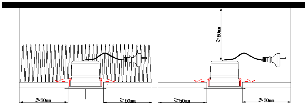
Installation clearance with ceiling insulation
